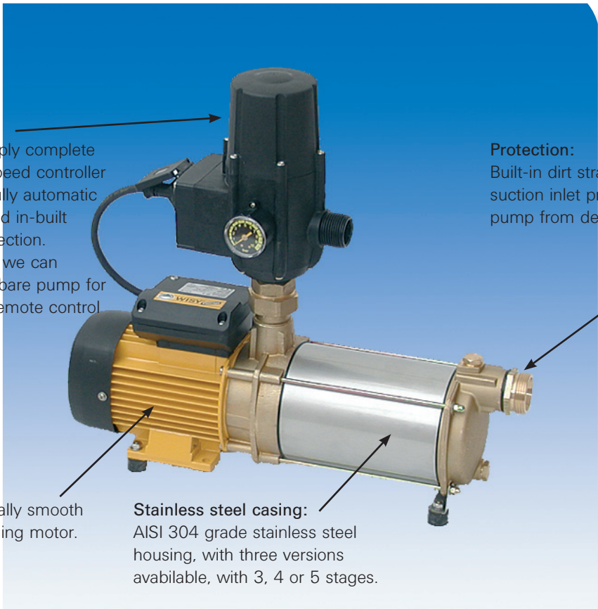
Aspri pump with Controlmatic automatic controller
