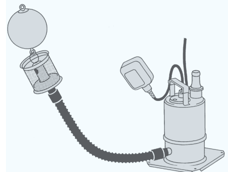
Provedo-Doc transfer pump with float switch and floating suction filter
