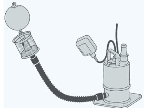
Provedo-Doc transfer pump with float switch and floating suction
